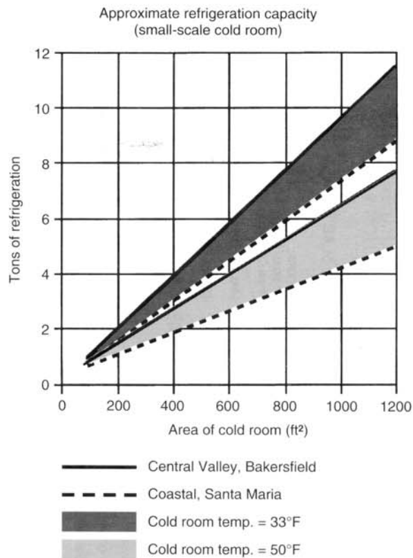
Figure 7. Approximate refrigeration capacity for small-scale cold rooms.
