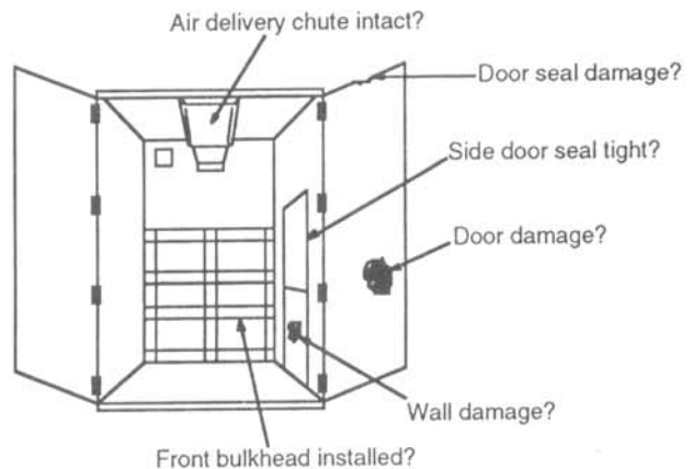
Figure 4. Factors to consider when inspecting a used trailer for purchase as a cold room.
